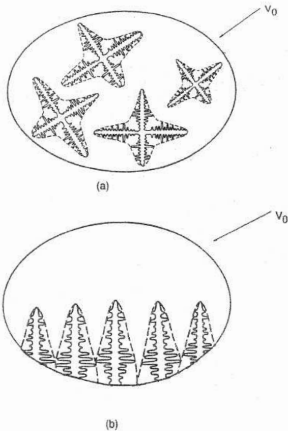
Figure 9 Schematic illustration of the averaging volume and the dendrite envelopes for: (a) equiaxed growth and (b) columnar growth.
