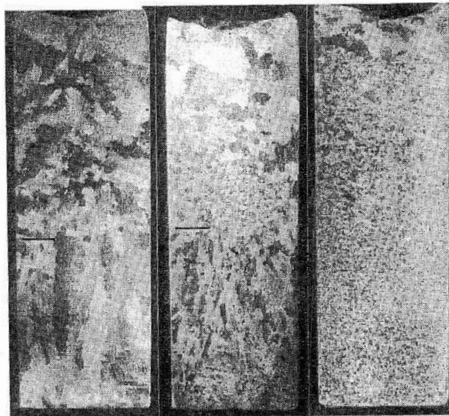
Figure 5 Grain structure of a vertically solidified Al-3 wt% Cu alloy slowing the columnar-to-equiaxed transition: (a) effect of increasing heat transfer coefficient (from left to right) and (b) effect of increasing grain refiner concentration (from left to right) [25].
