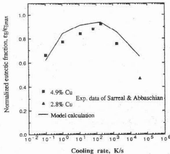
Figure 17 Effect of cooling rate on the eutectic fraction. Comparison of the present predictions with Sarreal and Abbaschian's experiments [74] (from Reference [40]).
