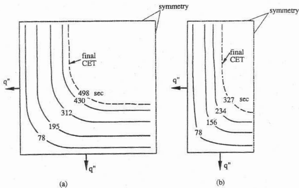
Figure 22 Evolution of the interface between the columnar and equiaxed zones in (a) 100 \times 100 mm square and (b) 50 \times 100 mm rectangular castings of an Al-3 wt% Cu alloy ( h = 65 \text{ W/m}^2\text{K} , n = 10^5 \text{ m}^{-3} and \Delta T_0 = 20 \text{ K} ). The dashed line denotes the final CET position [24].
