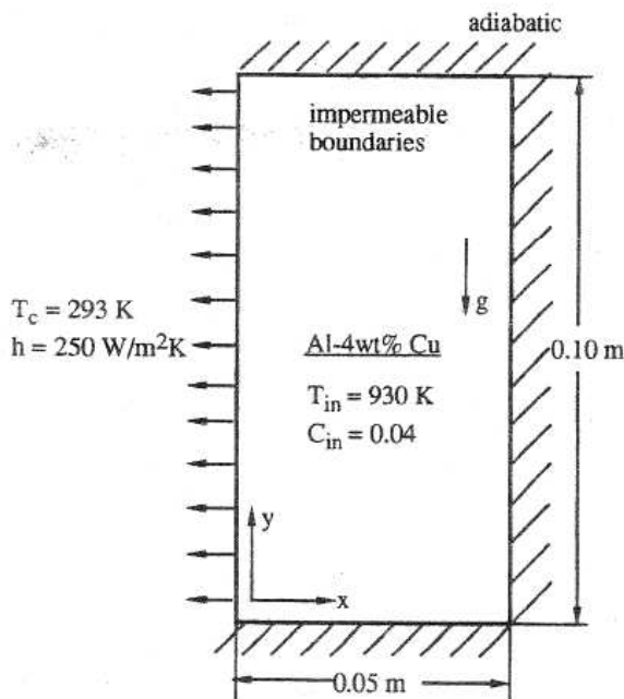
Figure 33 Schematic of the physical system used in the simulation of equiaxed dendritic solidification with convection.
