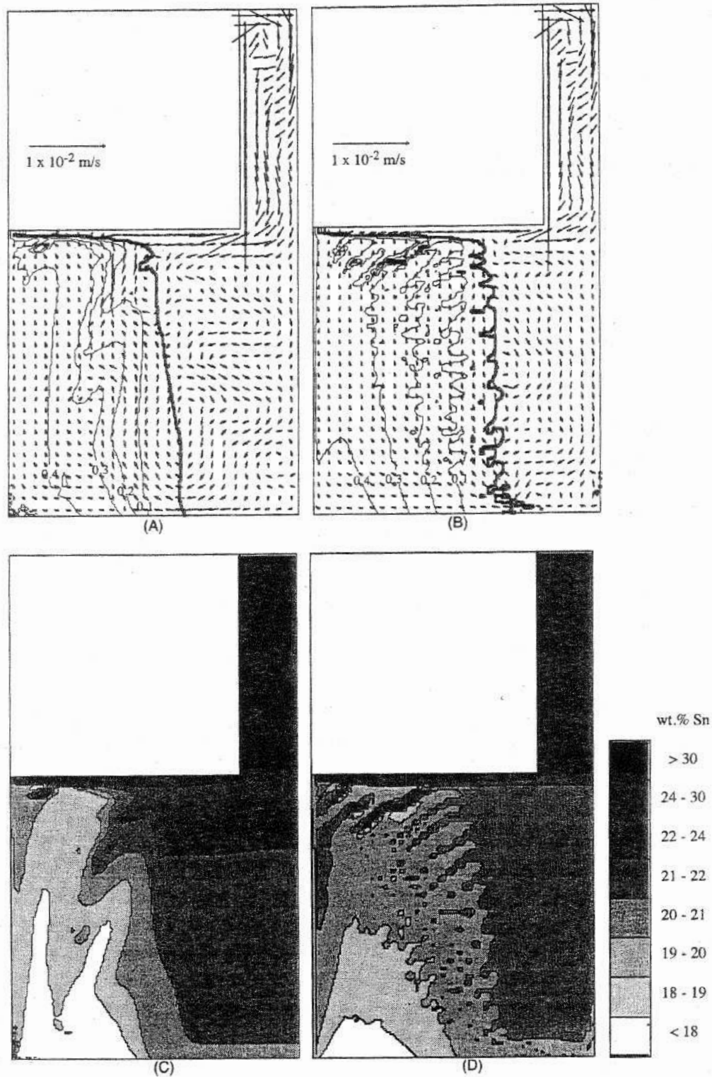
Figure 28 Velocity field, solid fraction isopleths and macrosegregation distributions after 250 s for the solidification of a Pb-20 wt% Sn alloy [93]: (a) Velocity field and solid fraction distribution using an anisotropic permeability model. (b) Velocity field and solid fraction distribution using an isotropic permeability model. (c) Macrosegregation pattern using an anisotropic permeability model. (d) Macrosegregation pattern using an isotropic permeability model.
