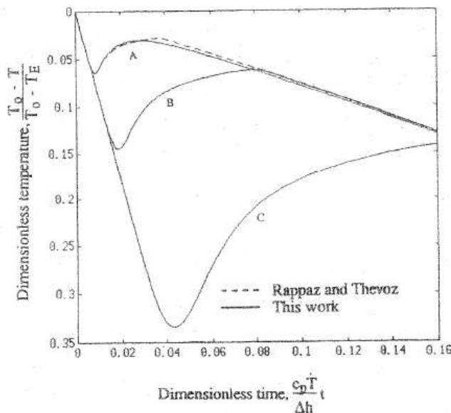
Figure 18 Comparisons of cooling curves for equiaxed dendritic growth, as predicted by the present model (solid lines) and Rappaz and Thevoz [34] (dashed lines) for final grain radii of (A) 100 \mu\text{m} , (B) 1 mm and (C) 10 mm [40].
