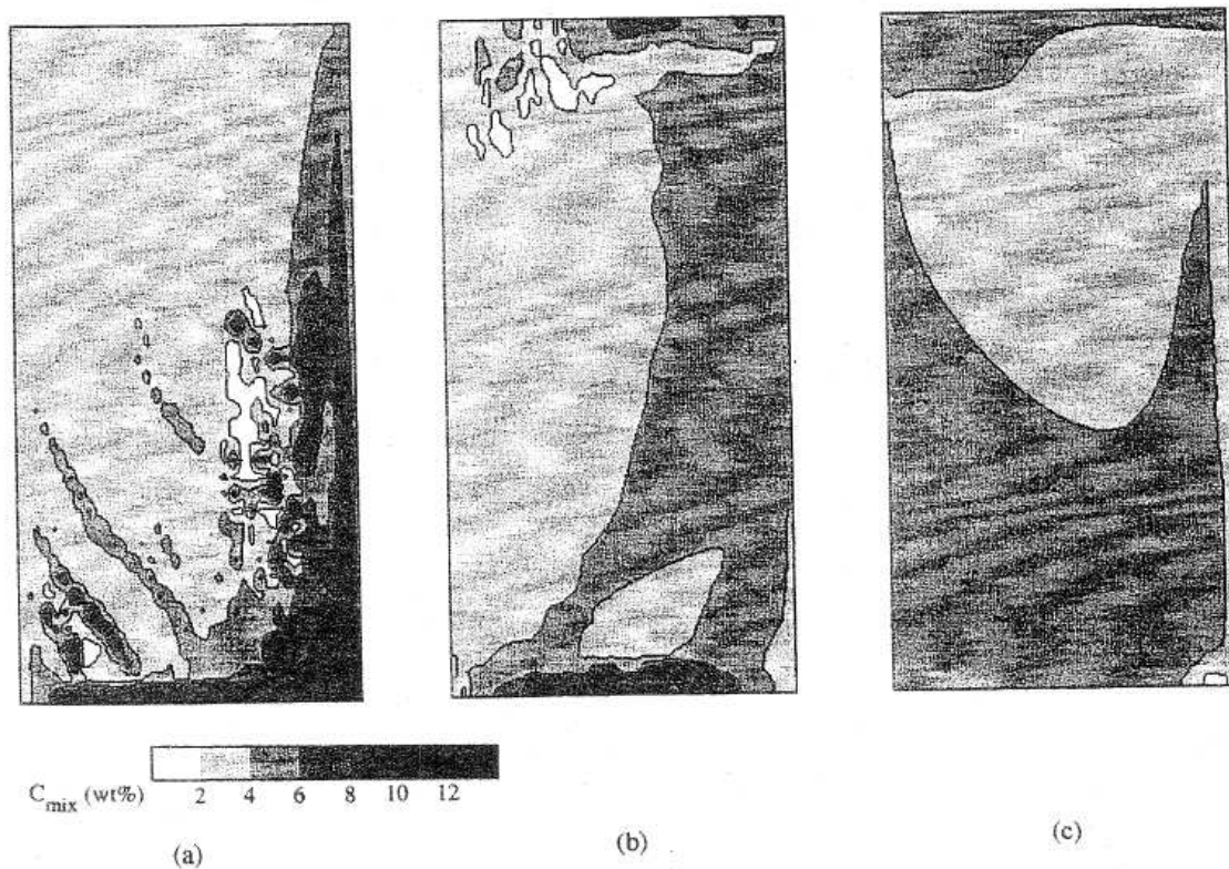
Figure 37 Final macrosegregation patterns for: (a) a stationary solid ( n_0 = 10^9 \text{ m}^{-3} ), (b) moving solid ( n_0 = 10^9 \text{ m}^{-3} ), and (c) moving solid ( n_0 = 10^{11} \text{ m}^{-3} ) [41].
