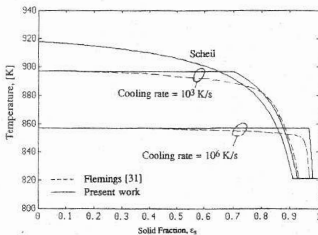
Figure 15 Effect of dendrite tip undercooling on the temperature vs solid fraction relation for columnar solidification of an Al-4.5 wt% Cu alloy [40].
