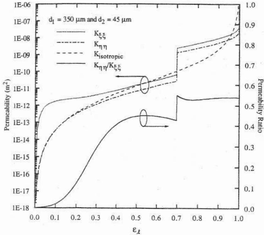
Figure 27 Variation of the permeabilities perpendicular, K_{\eta\eta} , and parallel, K_{\xi\xi} , to the primary dendrite arms for typical primary, d_1 , and secondary, d_2 , dendrite arm spacings, as well as for an approximate isotropic permeability. Also shown is the variation of the ratio of the perpendicular and parallel permeabilities with the liquid fraction.
