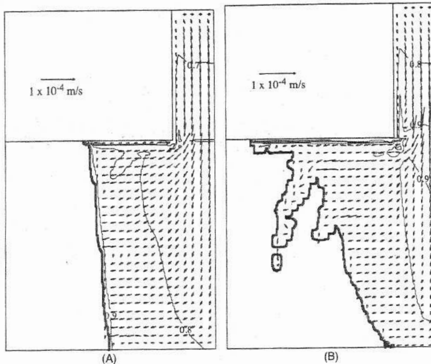
Figure 29 Velocity field and solid fraction isopleths near the end of solidification of a Pb-20 wt% Sn alloy [93]: (a) After 800 s assuming no microscopic solid species diffusion. (b) After 2050 s assuming complete microscopic solid species diffusion.
