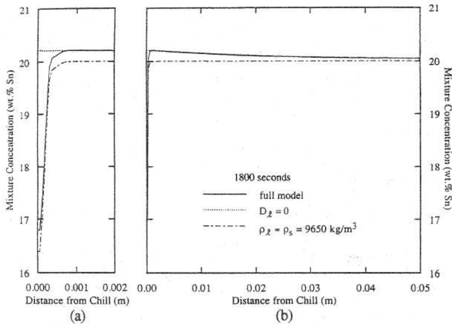
Figure 30 Macrosegregation profiles for the unidirectional solidification of a Pb-20 wt% Sn alloy with no buoyancy driven flow: (a) near the chill and (b) throughout the casting [93].
