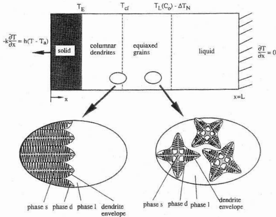
Figure 19 Schematic of the physical problem and illustration of the multiphase approach used in the CET simulations.
