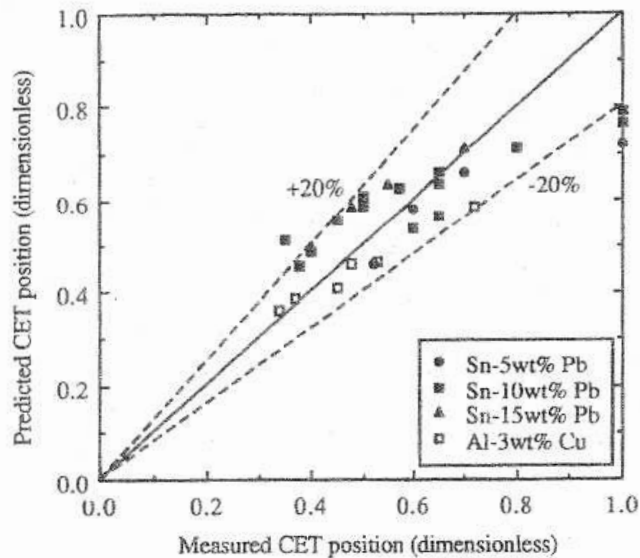
Figure 24 Comparison of the predicted CET positions with all experimental data reported in References 25, 82 (Sn-Pb alloys: n = 10^7 \text{ m}^{-3} , Al-3 wt% Cu alloy: n = 10^5 \text{ m}^{-3} ) [24].
