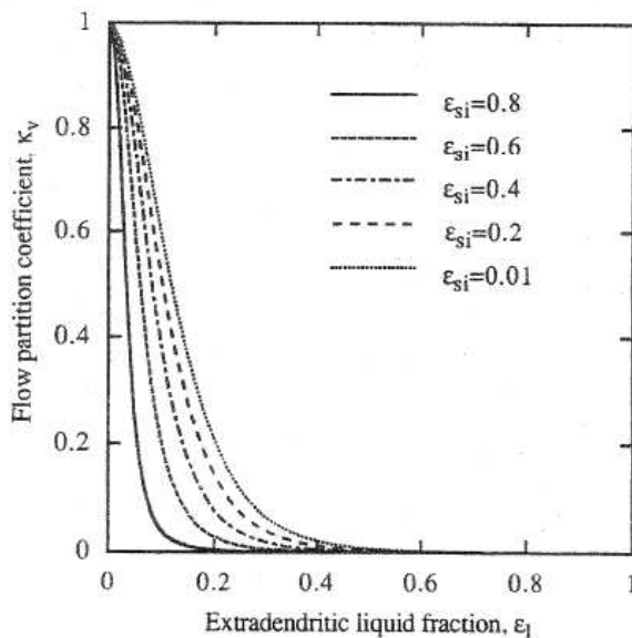
Figure 32 Flow partition coefficient as functions of the extradendritic liquid fraction and internal solid fraction for S_s/S_e = 0.1 [126].
