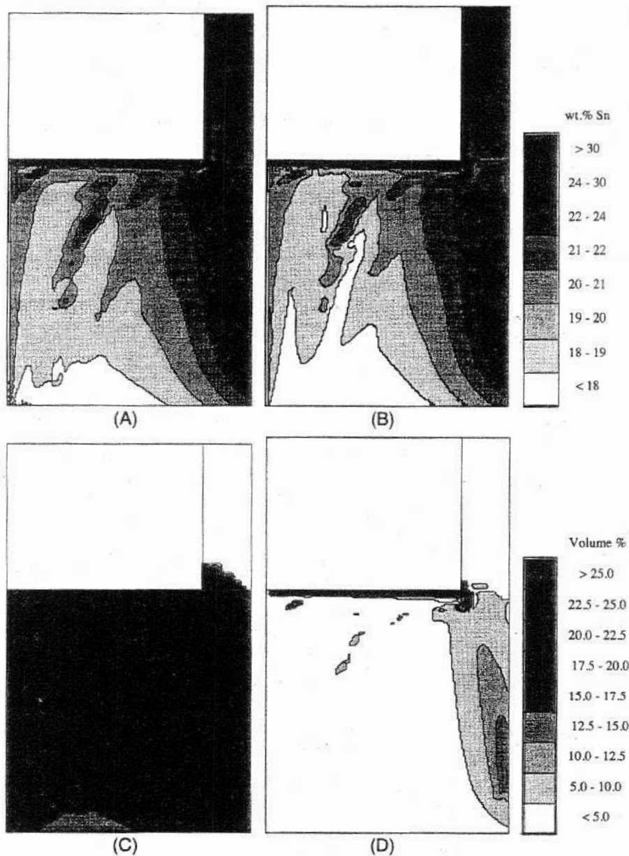
Figure 26 Final macrosegregation and eutectic fraction patterns for the solidification of Pb-20 wt% Sn alloy [93]: (a) Macrosegregation with no microscopic solid species diffusion. (b) Macrosegregation with complete microscopic solid species diffusion. (c) Eutectic fraction with no microscopic solid species diffusion. (d) Eutectic fraction with complete microscopic solid species diffusion.
