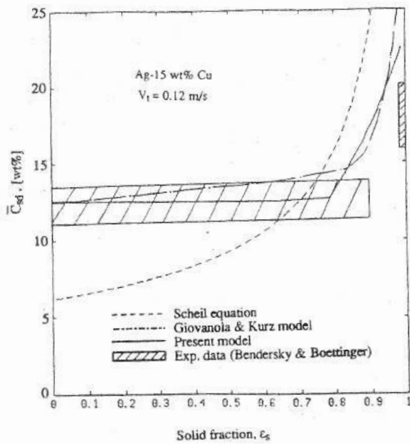
Figure 16 Comparisons of the present prediction of microsegregation in a rapidly solidified Ag-15 wt% Cu alloy with the Giovanola and Kurz's calculation [37] and the experimental data by Bendersky and Boettinger [73] (from Reference [40]).
