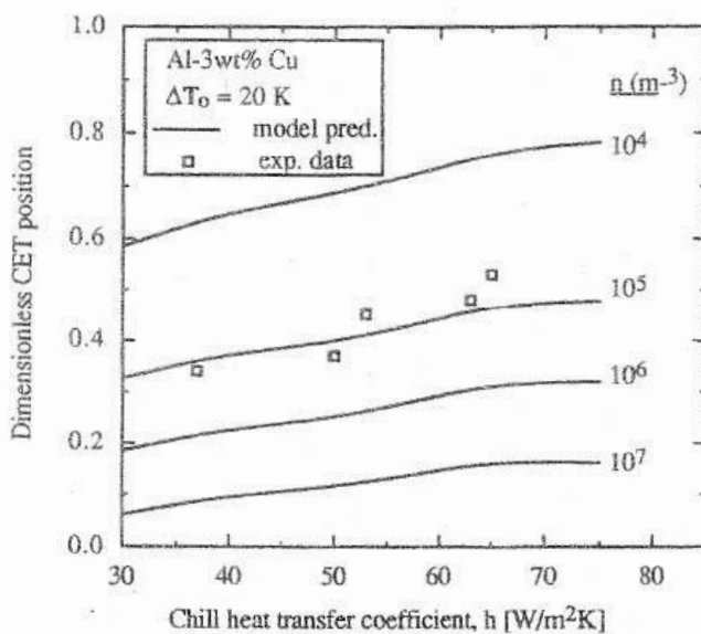
Figure 23 Effects of nuclei density and chill heat transfer coefficient on the CET position in a 1-D casting of an Al-3 wt% Cu alloy. Comparison with Ziv and Weinberg's data [25] (from Reference [24]).
