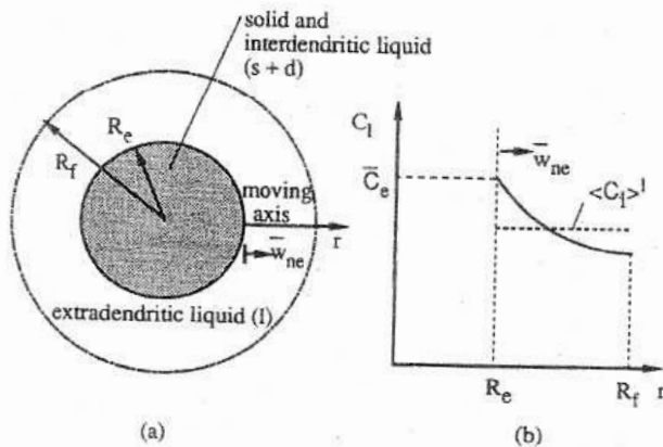
Figure 13 Equivalent sphere model for species diffusion in the extradendritic liquid: (a) geometry and (b) concentration profile.
