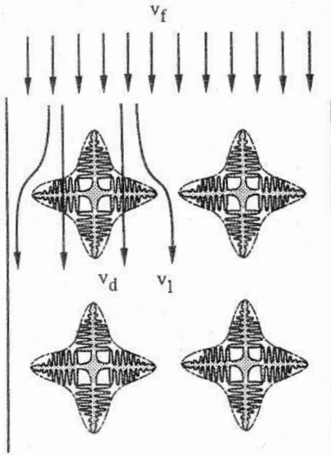
Figure 31 Schematic of the partitioning of the liquid flow through the interdendritic and extradendritic regions in equiaxed solidification.
