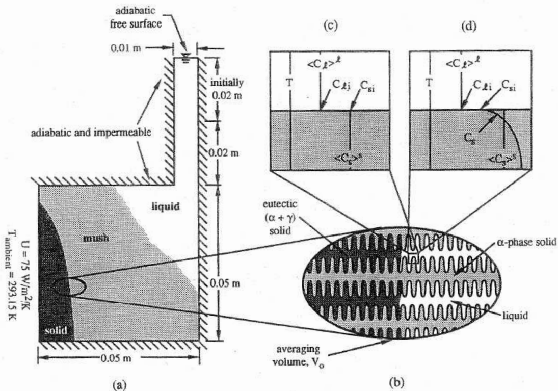
Figure 25 (a) Schematic illustration of the domain and boundary conditions used by Schneider and Beckermann [93] to simulate the solidification of a Pb-20 wt% Sn alloy. (b) A typical averaging volume that includes ( \alpha -phase solid, eutectic ( \alpha + \gamma ) solid, and liquid. (c) Schematic illustration of the assumed microscopic temperature and concentration profiles for the case of complete microscopic solid species diffusion. (d) Schematic illustration of the assumed microscopic temperature and concentration profiles for the case of no microscopic solid species diffusion.
