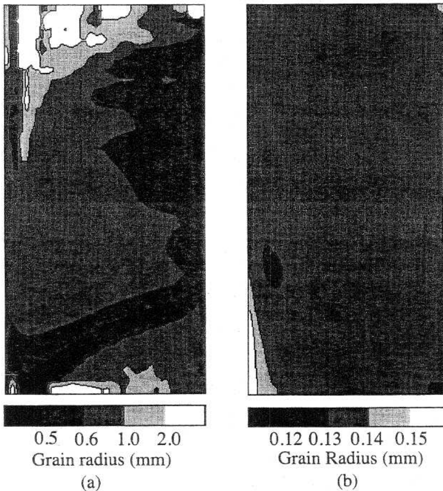
Figure 36 Predicted final grain size ( R_e ) distribution for (a) n_0 = 10^9 \text{ m}^{-3} , and (b) n_0 = 10^{11} \text{ m}^{-3} [41].
