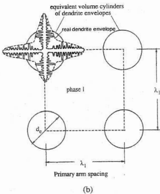
Figure 12 Schematic of shape factors for (a) an equiaxed dendritic envelope and (b) a square arrangement of columnar dendrite envelopes.
