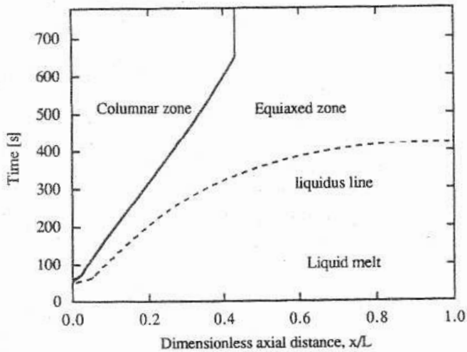
Figure 21 Map of different regions developing in a 1-D casting of an Al-3 wt% Cu alloy ( h = 65 \text{ W/m}^2\text{K} , n = 10^5 \text{ m}^{-3} and \Delta T_o = 20 \text{ K} ) [24].
