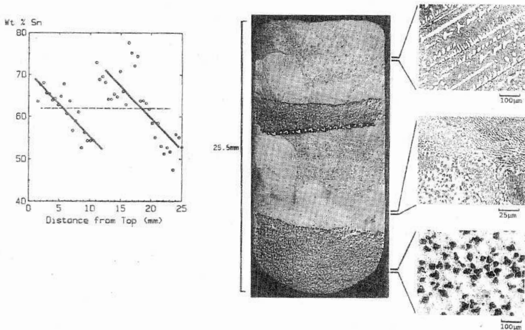
Figure 8 Effect of settling of equiaxed grains on solidification of an undercooled Pb-Sn eutectic alloy with a stainless steel screen near the center. (Left) microprobe composition measurements. (Center and right) micrographs of longitudinal cross-sections [30].
