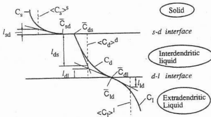
Figure 10 Illustration of the species diffusion lengths.
