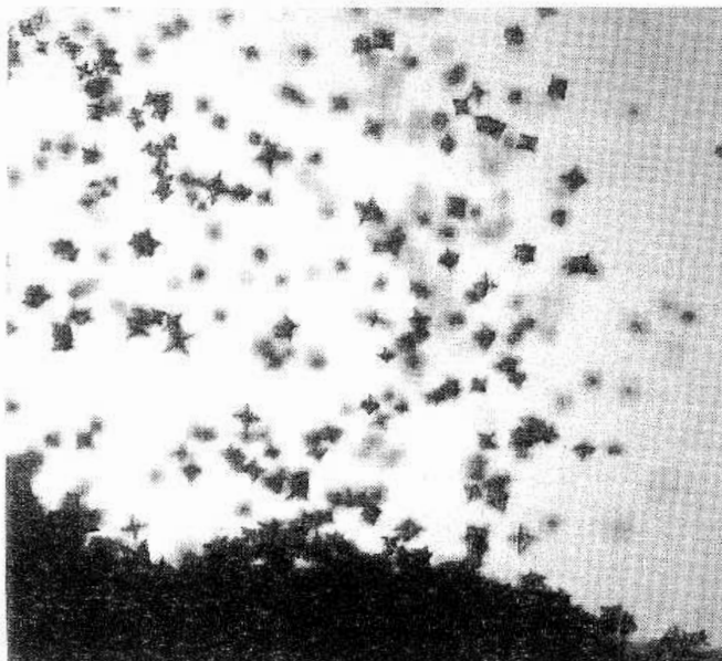
Figure 4 Equiaxed solidification of a \text{NH}_4\text{Cl-H}_2\text{O} solution: (a) shadowgraph image and (b) close-up of sedimenting crystals [21].
