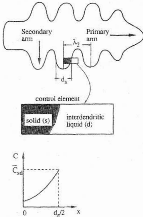
Figure 11 One-dimensional, plate-like model of a dendrite arm and illustration of the solid concentration profile.
