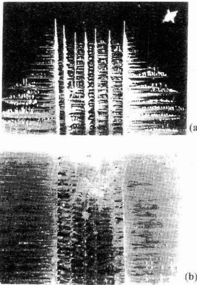
Figure 3 Channel formation in a columnar dendritic mushy zone: (a) mouth of the channel, and (b) 8 to 10 mm lower in the mushy zone [20].
