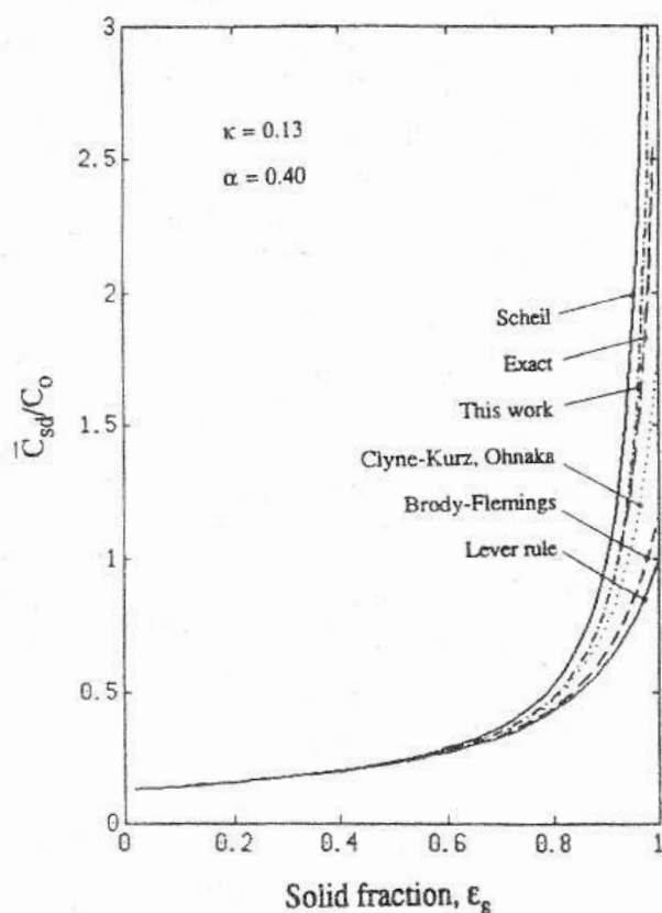
Figure 14 Microsegregation of P in \delta -Fe, as predicted by various solute diffusion models [40].
