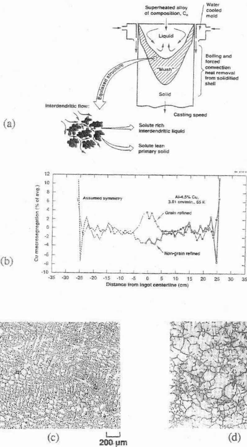
Figure 6 Effects of grain refining on macrosegregation in an Al-4.5 wt% round ingot: (a) schematic of the continuous casting apparatus, (b) comparison of the macrosegregation profiles, (c) non-grain-refined microstructure, and (d) grain-refined microstructure [27].
