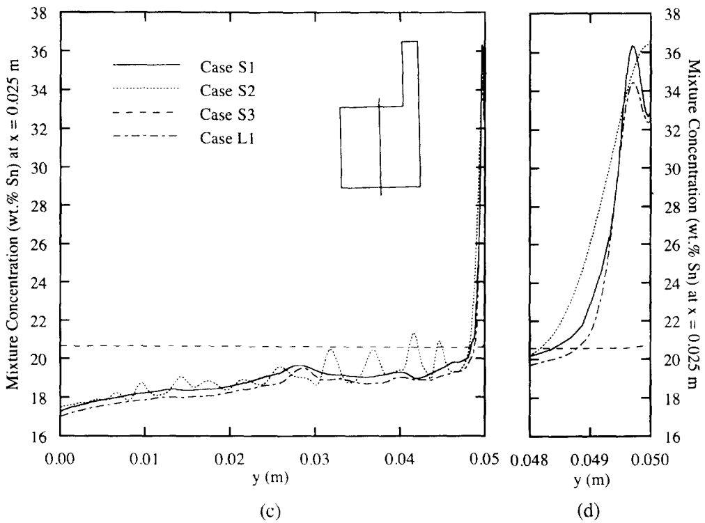
Fig. 8. Final macrosegregation profiles : (a) and (b) along y = 0.025 m, and (c) and (d) along x = 0.025 m.
