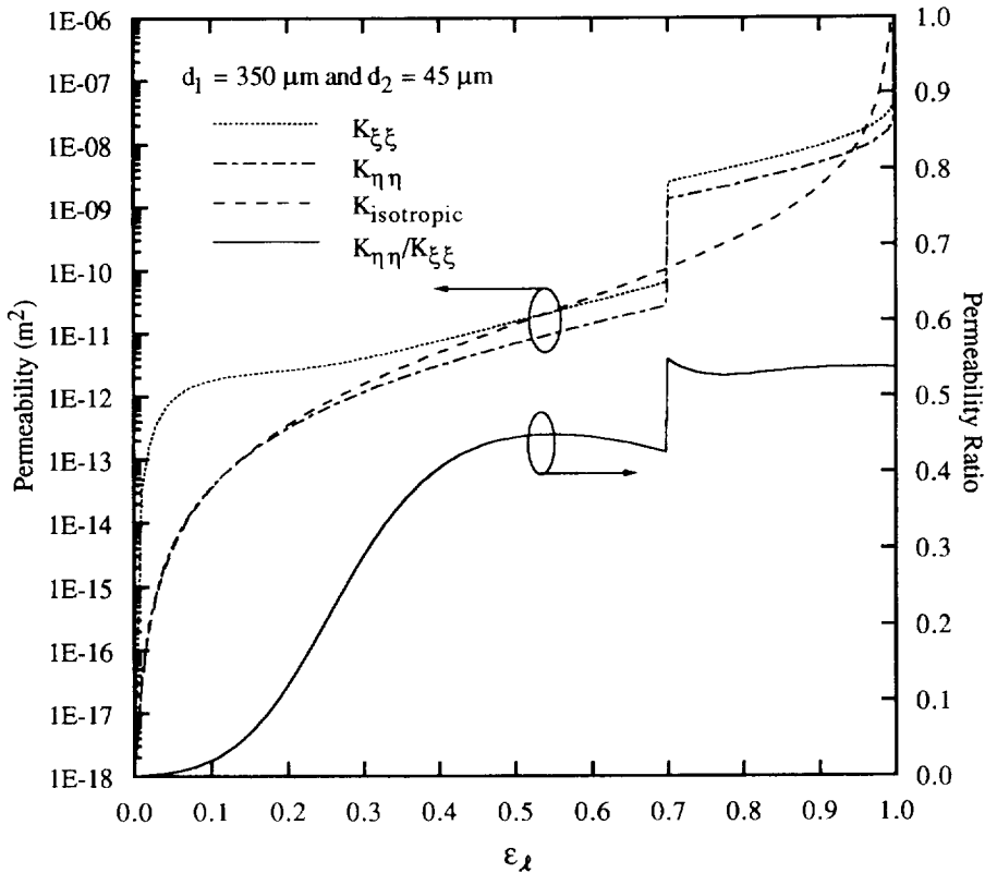
Fig. 2. Variation with liquid fraction of the permeabilities perpendicular, K_{\eta\eta} , and parallel, K_{\xi\xi} , to the primary dendrite arms, and of the approximate isotropic permeability. Also shown is the variation of the ratio of the perpendicular and parallel permeabilities.
