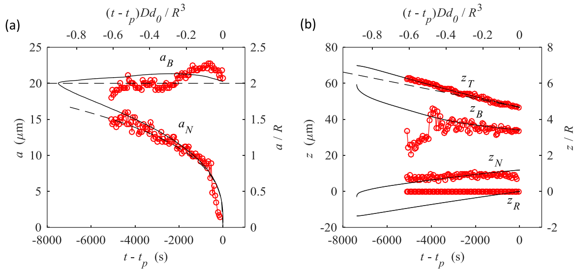
Fig. 8. Evolution of geometrical parameters for Sidearm 2; red circles: experimental measurements, black lines: numerical model; bottom and left axes are in physical units, top and right axes in scaled units, respectively; (a) bulge and neck diameter [dashed line in a_B : reference radius R = a_B/2 for the model, dashed line in a_N : fit according to Eq. (1)]; (b) vertical positions for tip, bulge, neck and root [dashed line in z_T : analytical model Eq. (10)]. (For interpretation of the references to colour in this figure legend, the reader is referred to the Web version of this article.)
