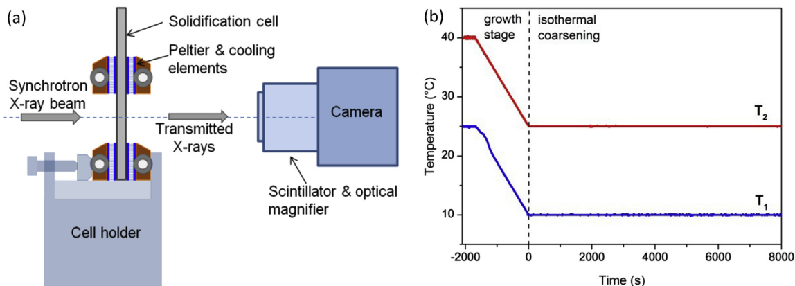
Fig. 1. (a) Schematic of the experimental setup showing the arrays of Peltier elements (bottom cooler and top heater). The thermocouples T_1 and T_2 were positioned at distances of 1 and 16 mm, respectively from the upper edge of the cooler. (b) Thermal regime: blue line ( T_1 ) – temperature curve near the cooler; red line ( T_2 ) – temperature curve near the heater. (For interpretation of the references to colour in this figure legend, the reader is referred to the Web version of this article.)
